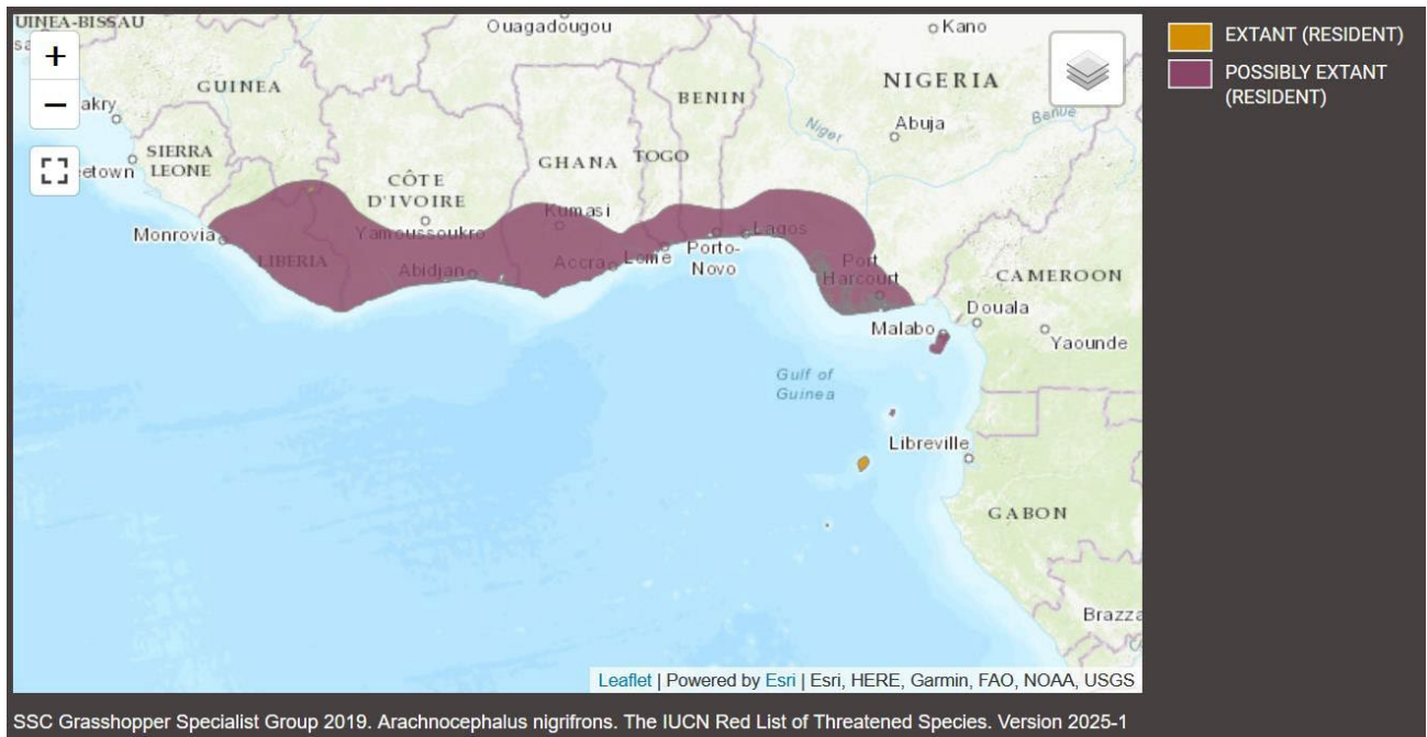
Figure 76. Range of Arachnocephalus nigrifrons (IUCN, 2025-I)
