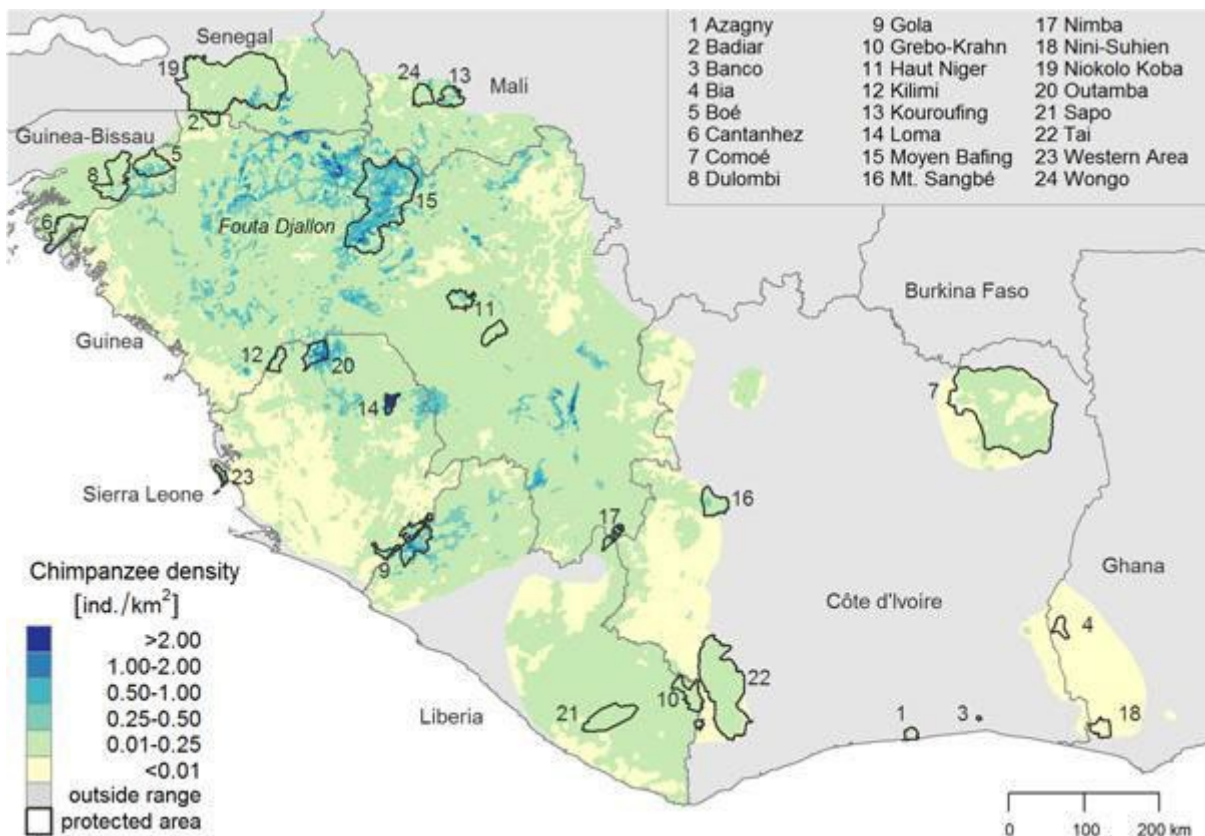
Figure 33. Modeled western chimpanzee density distribution (Heinicke et al., 2019)
