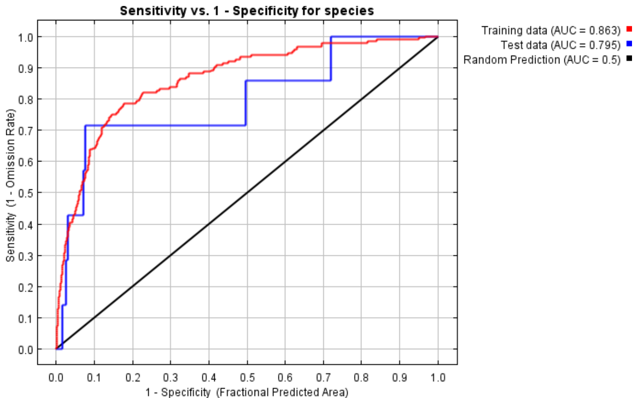
Figure 24. Evaluation results of the climatic habitat suitability of the Pygmy Hippopotamus in Liberia (FinnOC, 2025)
