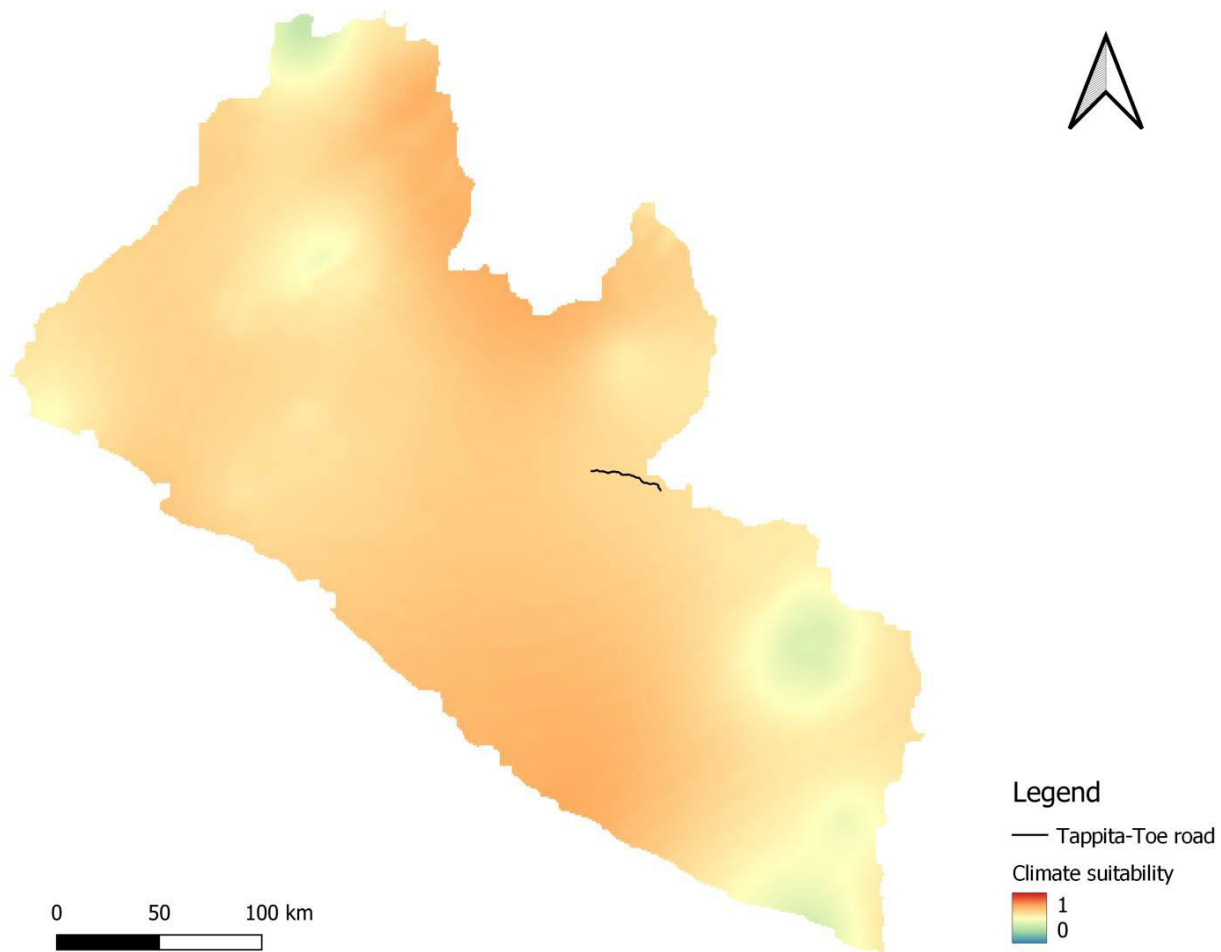
Figure 29. Predicted climatic suitability of the White-bellied pangolin in Liberia (FinnOC, 2025)
