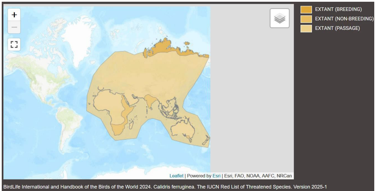
Figure 78. Range of Calidris ferruginea (IUCN, 2025-I)
