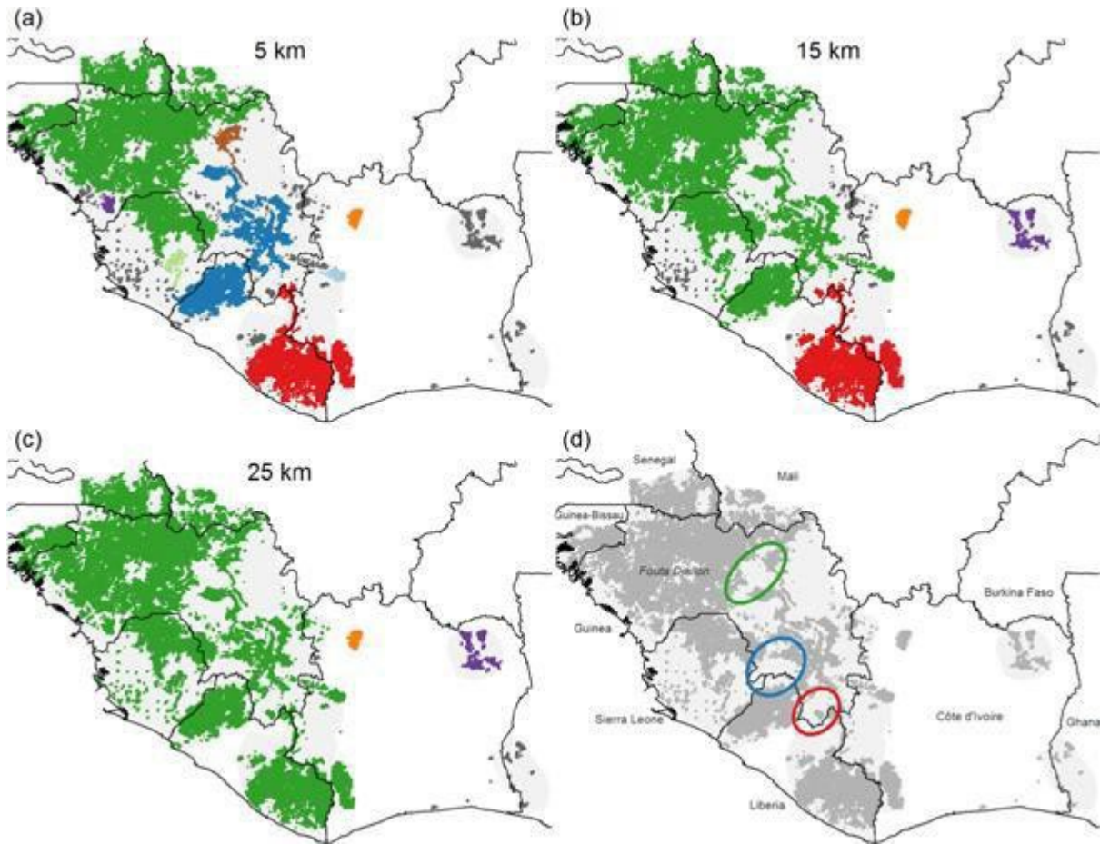
Figure 34. Scenarios for sub-populations based on three minimum distance thresholds(Heinicke et al., 2019)
