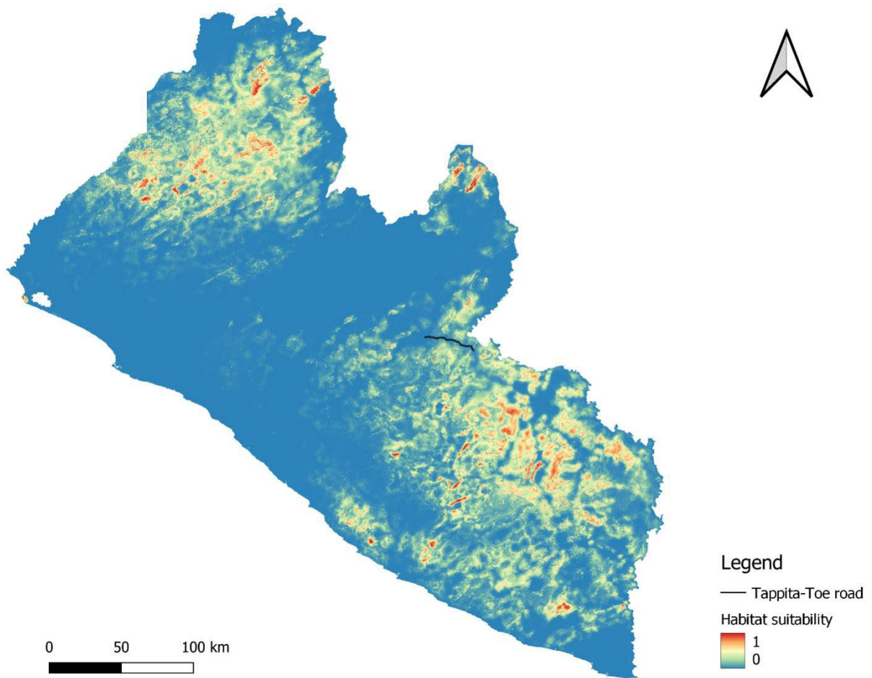
Figure 31. Potential distribution of chimpanzee populations in Liberia (Frazier et al, 2021)
