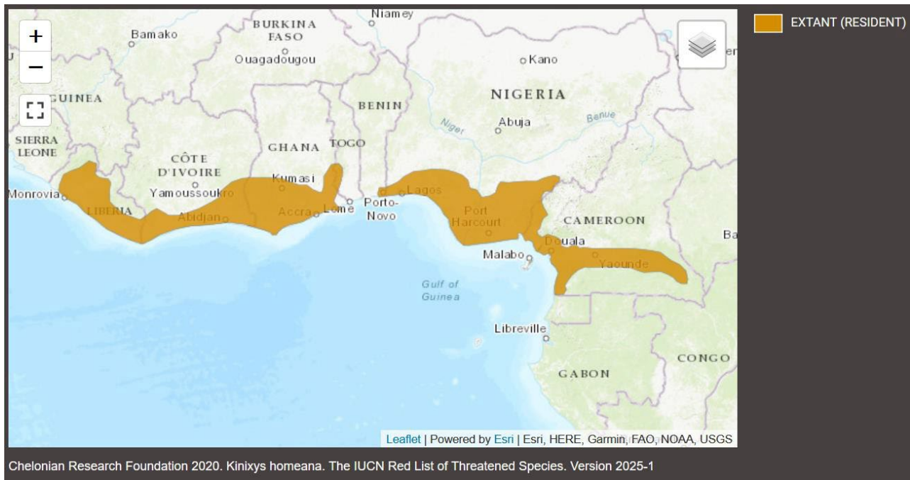
Figure 58. Range of Kinixys homeana (IUCN, 2025-I)
