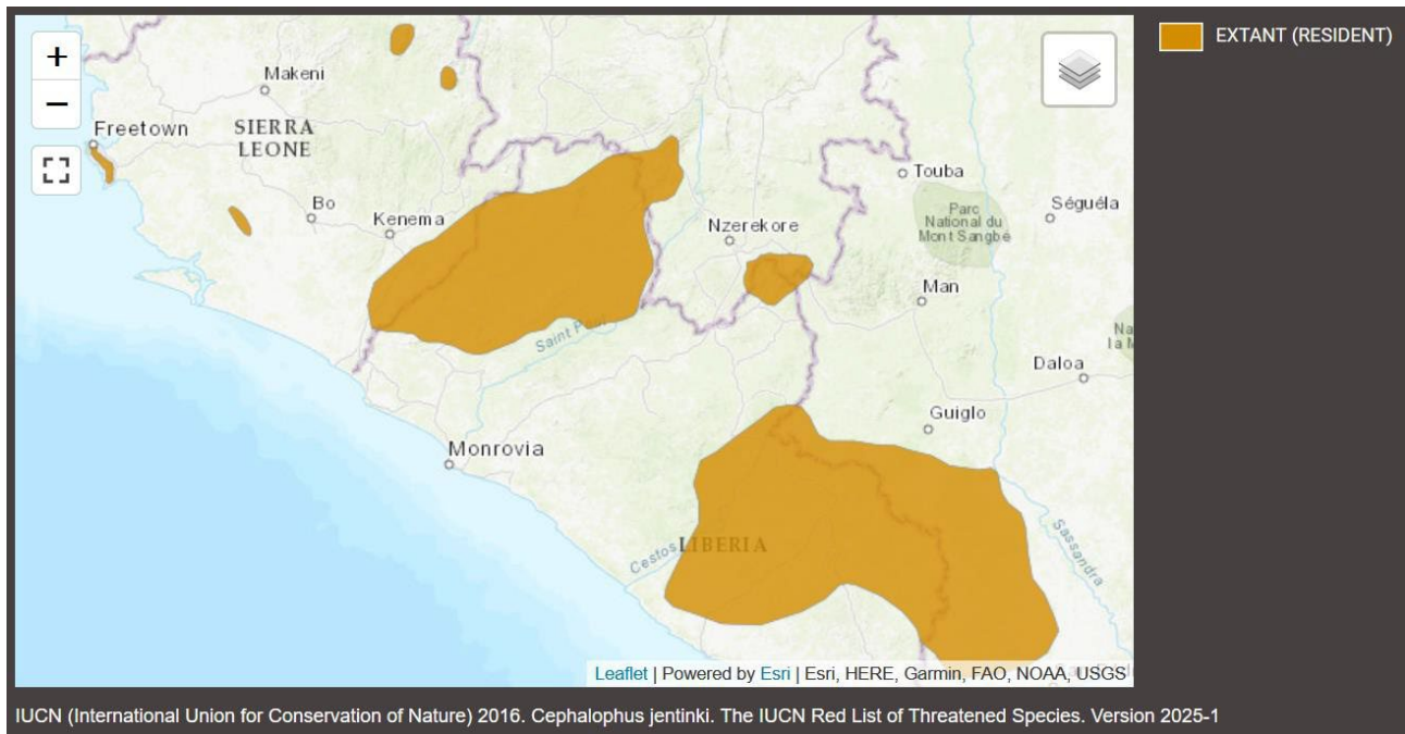
Figure 62. Range of Cephalophus jentinki (IUCN, 2025-I)
