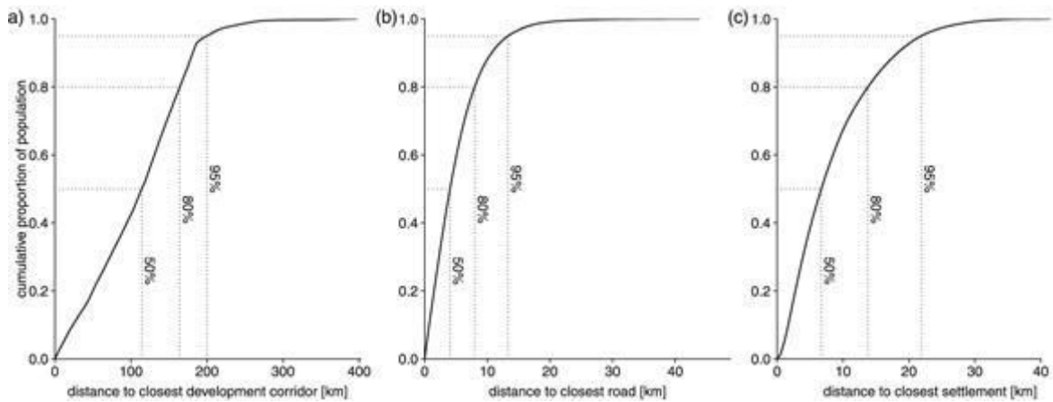
Figure 35. Cumulative proportion of western chimpanzees living within increasing distance to (a) 'development corridors', (b) roads, and (c) settlements. Plot (b) shows, for example, that 80% of western chimpanzees live less than 10 km from the nearest road (Heinicke et al., 2019)
