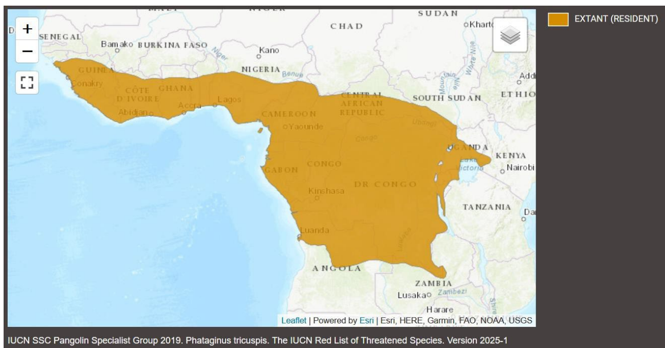
Figure 84. Range of Phataginus tricuspis (IUCN, 2025-I)
