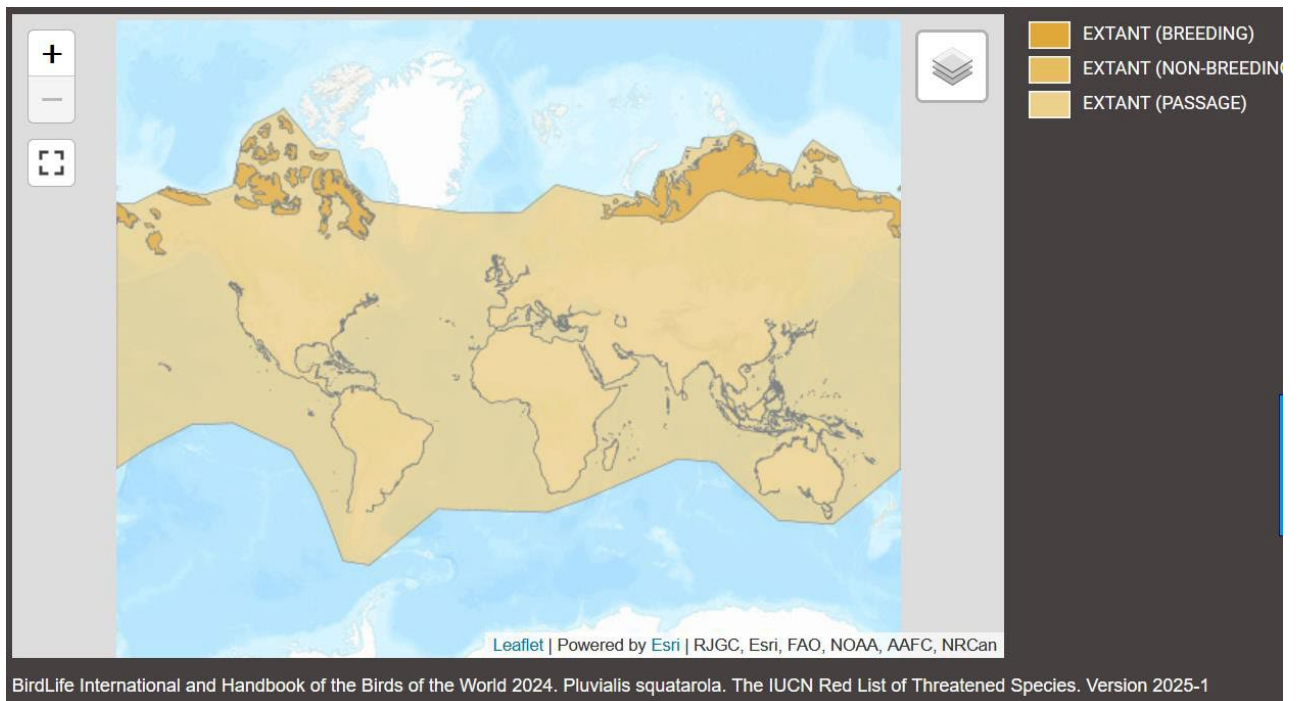
Figure 79. Range of Pluvialis squatarola (IUCN, 2025-I)
