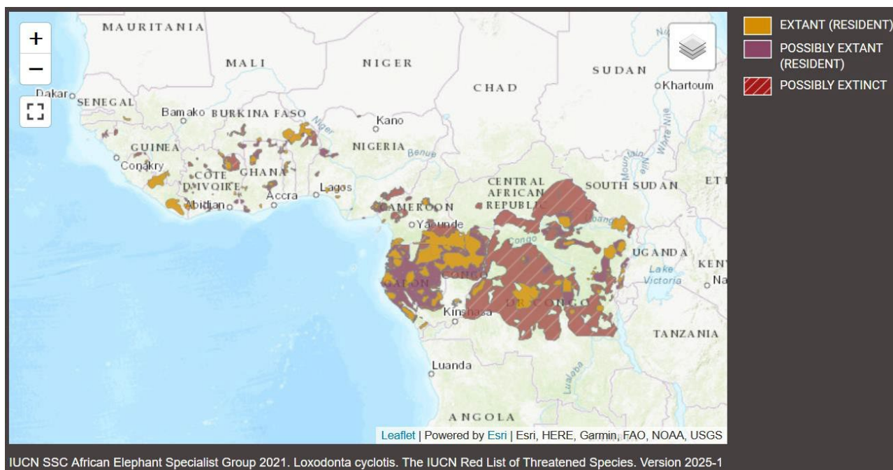
Figure 61. Range of Loxodonta cyclotis (IUCN, 2025-I)
