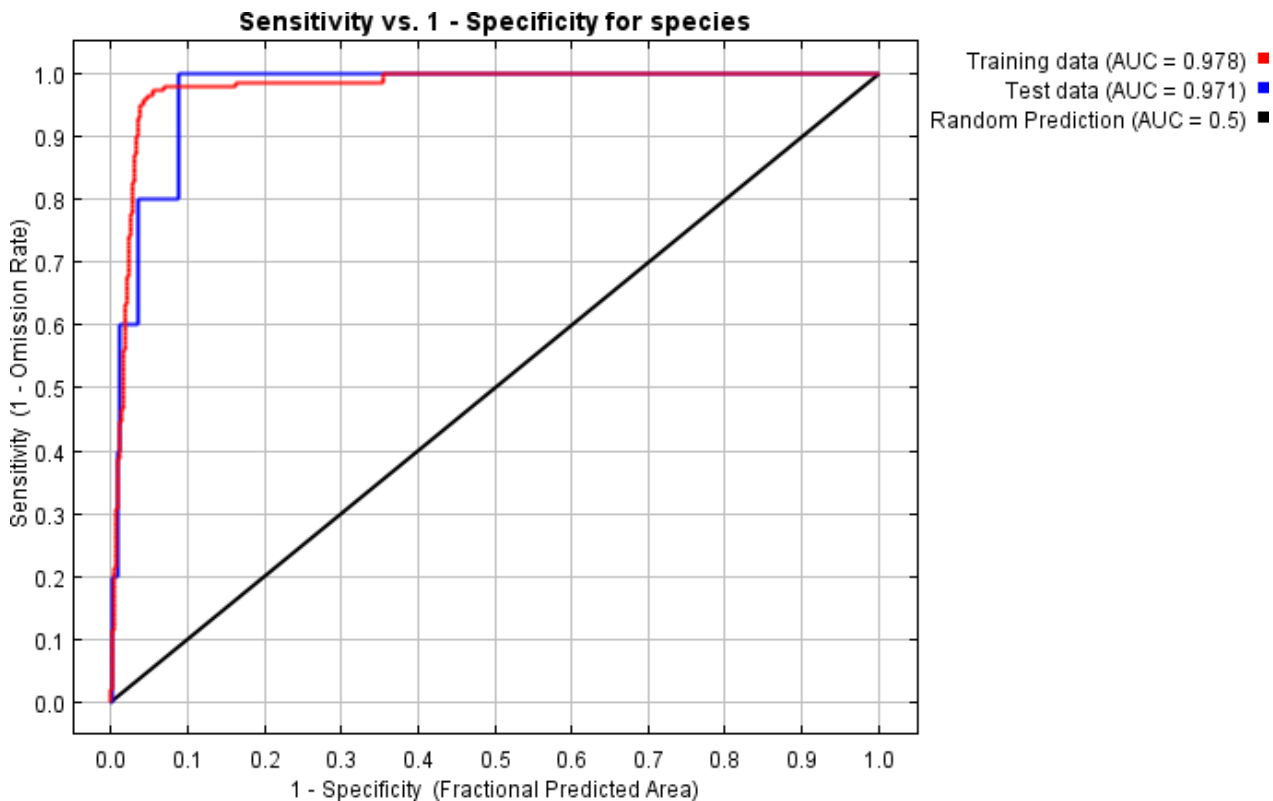
Figure 22. Evaluation results of the climatic habitat suitability of the African Forest Elephant in Liberia (FinnOC, 2025)
