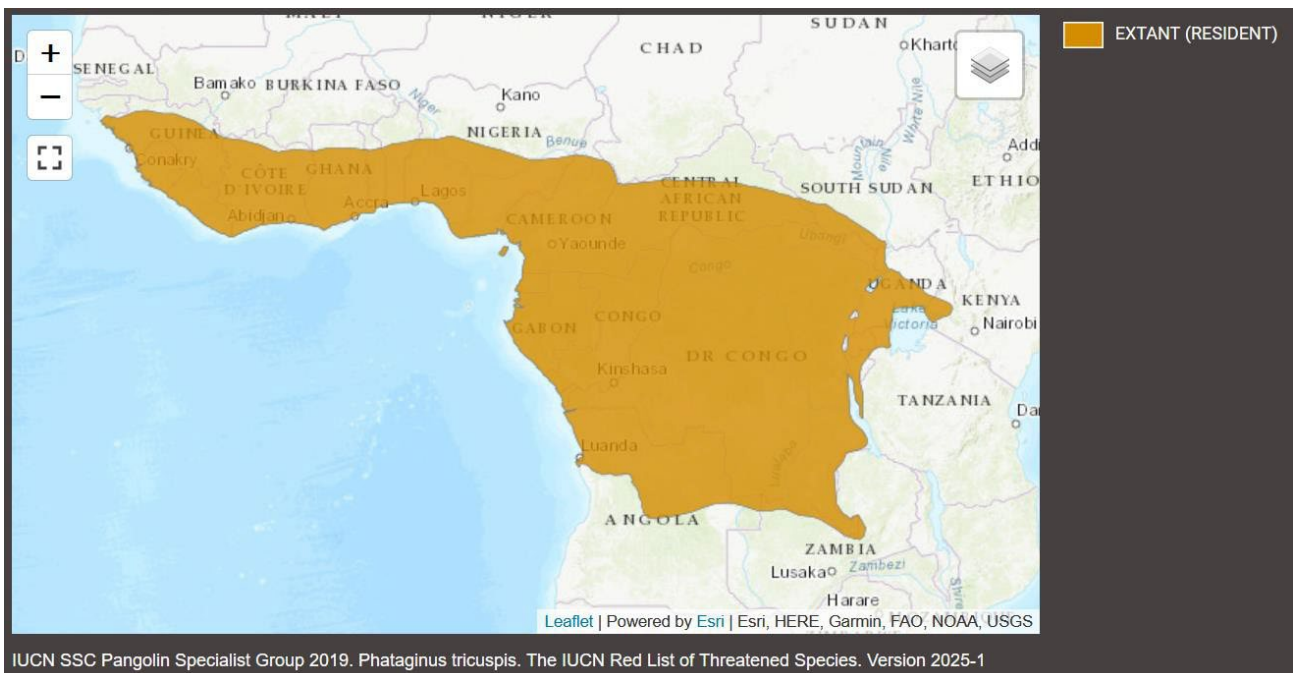
Figure 67. Range of Phataginus tricuspidis (IUCN, 2025-I)
