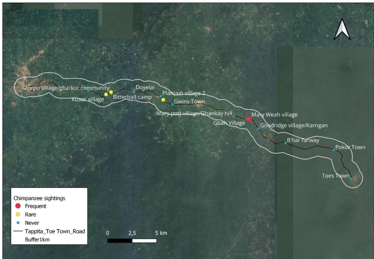
Figure 53. Community sightings of chimpanzee in the thick forest areas
