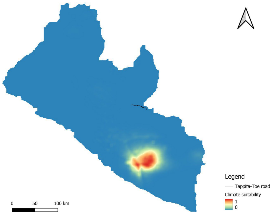
Figure 27. Predicted climatic suitability of the Giant pangolin in Liberia (FinnOC, 2025)
