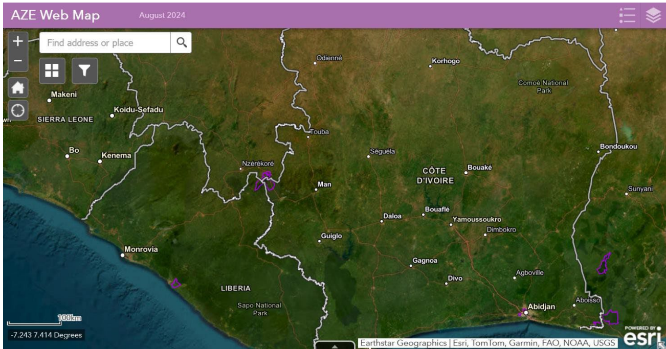
Figure 16. Alliance for Zero Extinction (AZE) areas in Liberia (AZE, 2024)
