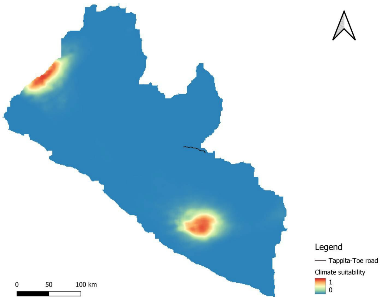
Figure 23. Predicted climatic suitability of the African Forest Elephant in Liberia (FinnOC, 2025)
