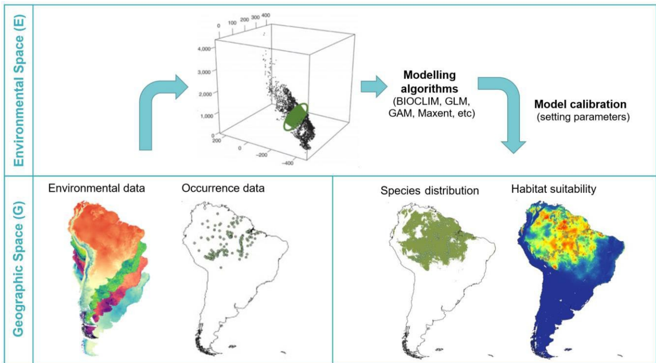
Figure 17. Example of methodological framework for modelling the distribution of species.
