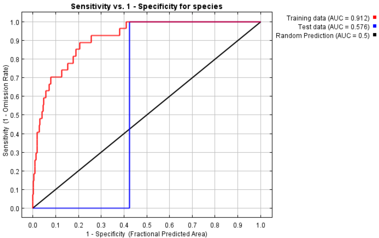
Figure 20. Evaluation results of the climatic habitat suitability of the Timnhed parrot in Liberia (FinnOC, 2025)
