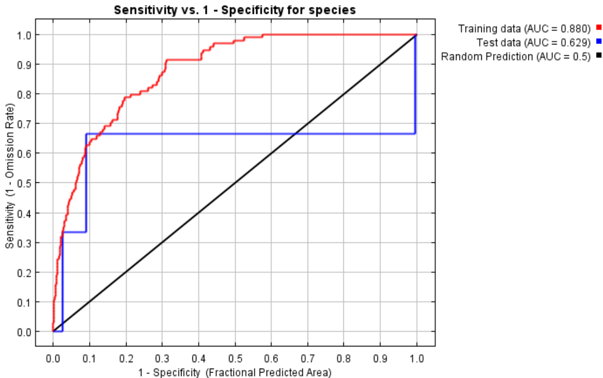
Figure 18. Evaluation results of the climatic habitat suitability of the Chimpanzees in Liberia (FinnOC, 2025)
