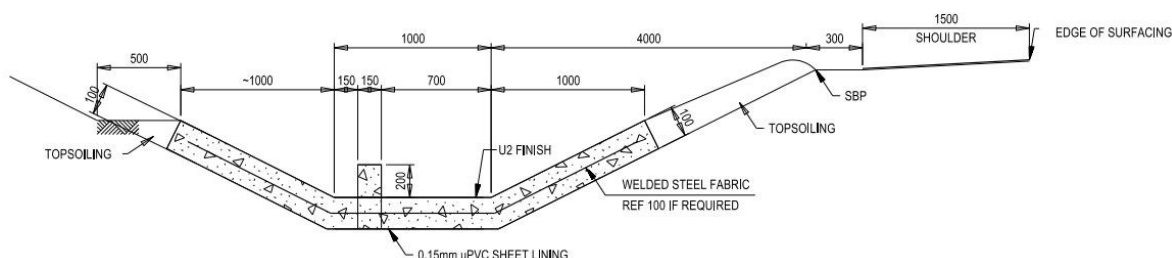
Figure 6. Proposed concrete side drain design. Source: AURECON (2020).
