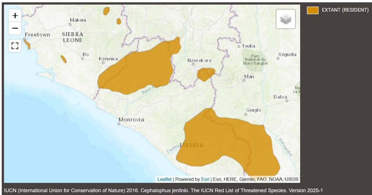
Figure 86. Range of Cephalophus jentinki (IUCN, 2025-I)
