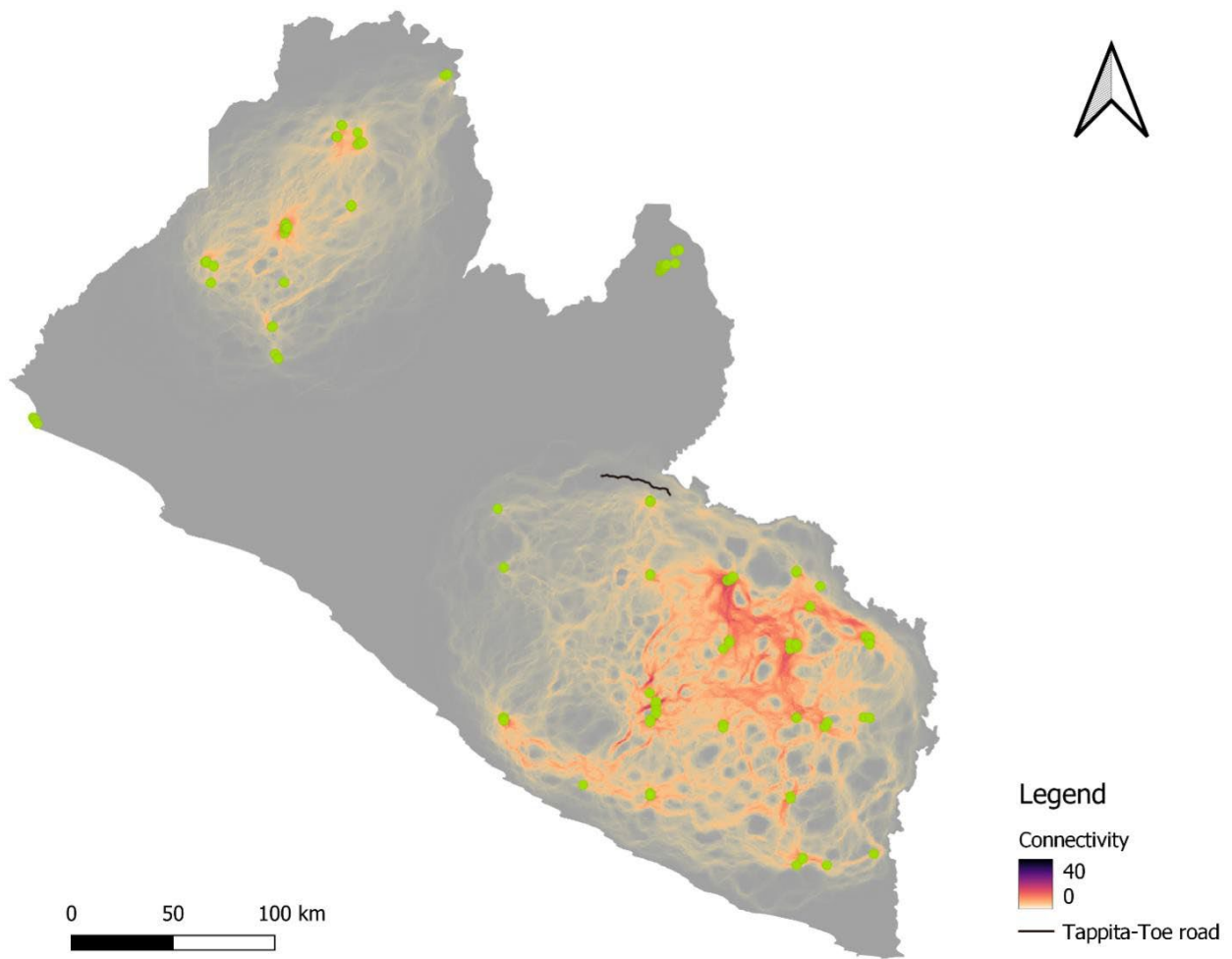
Figure 32. Connectivity analysis of chimpanzee populations in Liberia (Frazier et al, 2021). Green dots show the occurrence locations of chimpanzees in Liberia.
