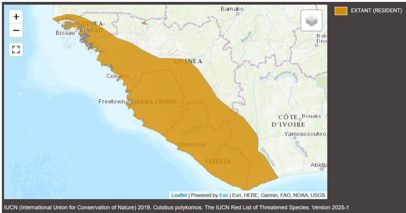
Figure 64. Range of Colopus polykomos (IUCN, 2025-I)
