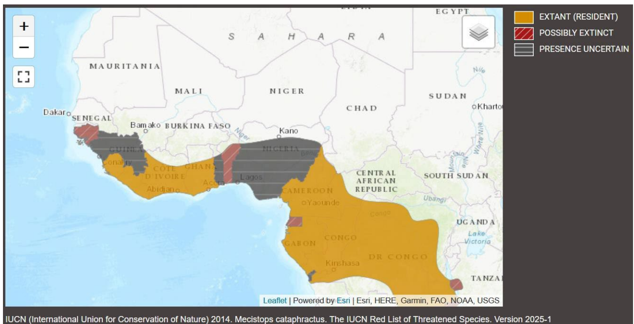
Figure 59. Range of Mecistops cataphractus (IUCN, 2025-I)
