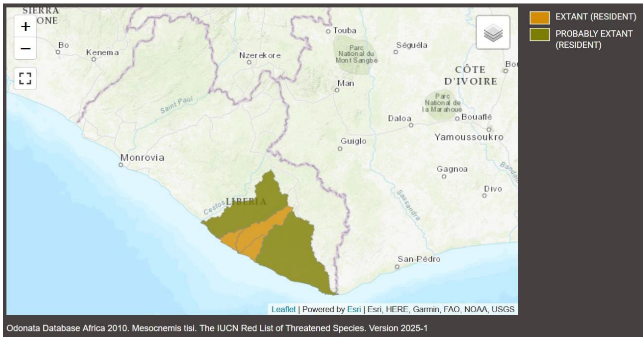
Figure 71. Range of Mesocnemis tisi (IUCN, 2025-I)
