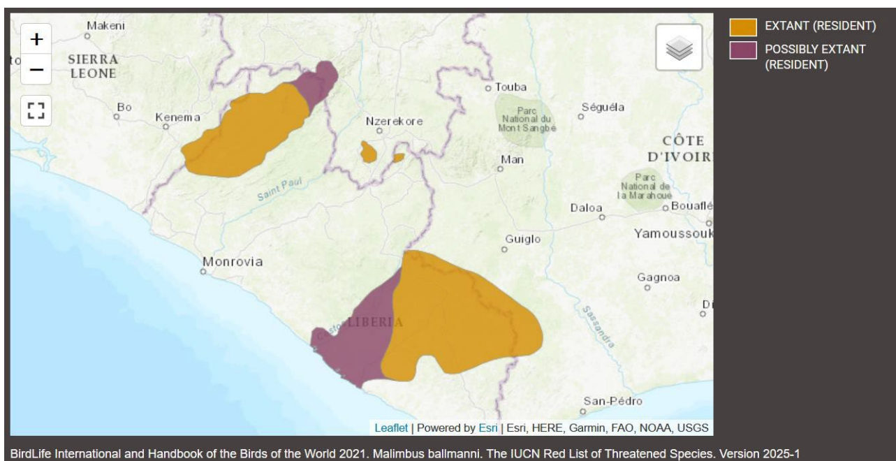
Figure 75. Range of Malimbus ballmanni (IUCN, 2025-I)
