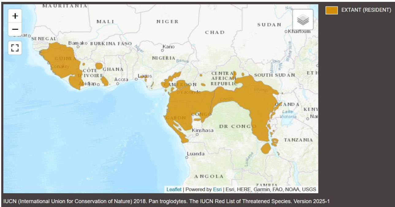
Figure 68. Range of Pan troglodytes (IUCN, 2025-I)
