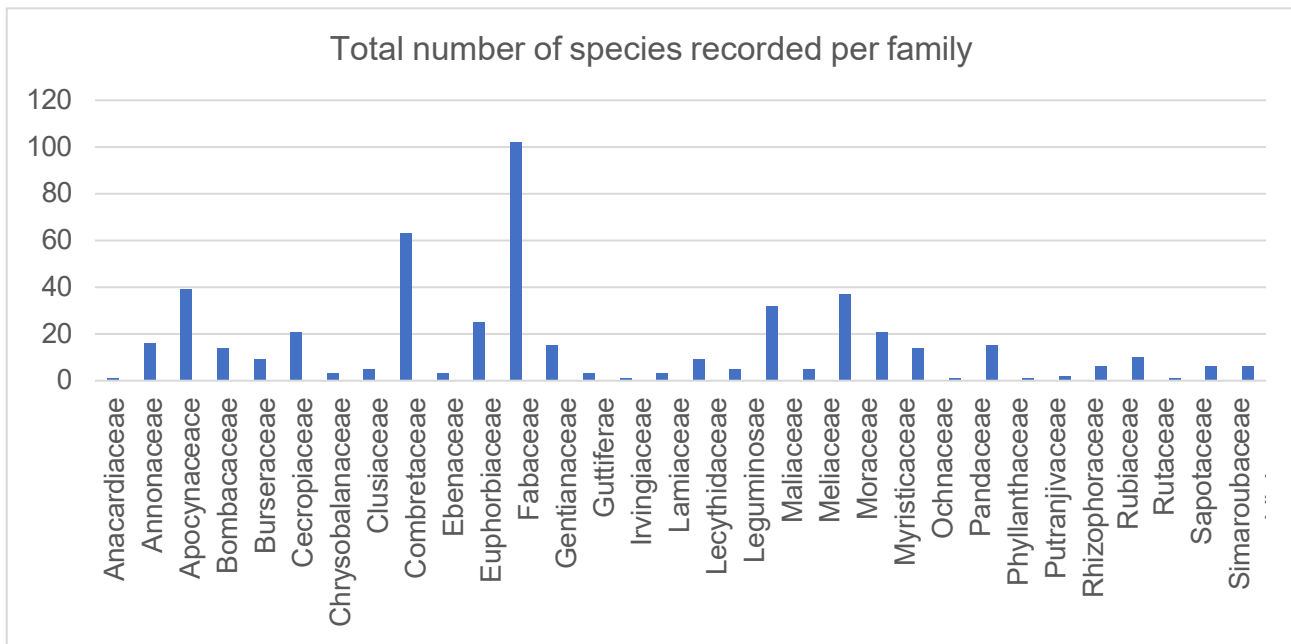
Figure 47. Graphical tabular presentation of the total number of flora species per family within the RETRAP Corridor 40 Km (Tappita-Toe Town).
