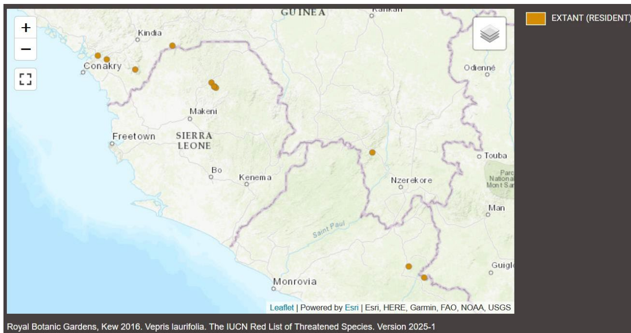
Figure 60. Range of Vepris laurifolia (IUCN, 2025-I)
