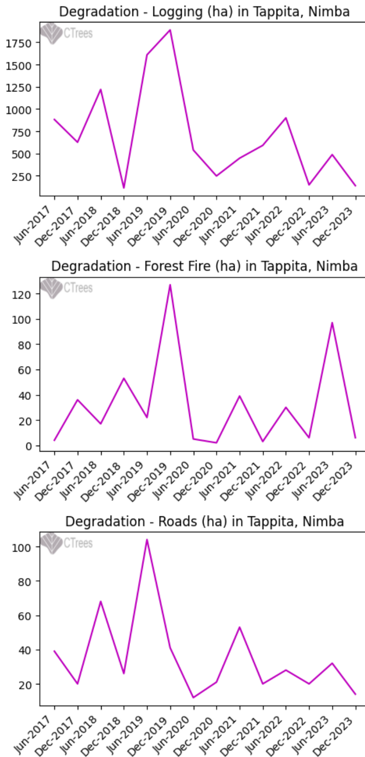
Figure 42. Deforestation and degradation in Nimba District (Source: REDD+ AI / Ctrees)
