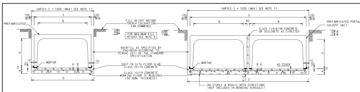
Figure 8. Proposed typical designs for single portal (left) and multiple portal (right) box culverts. Source: AURECON (2020).
