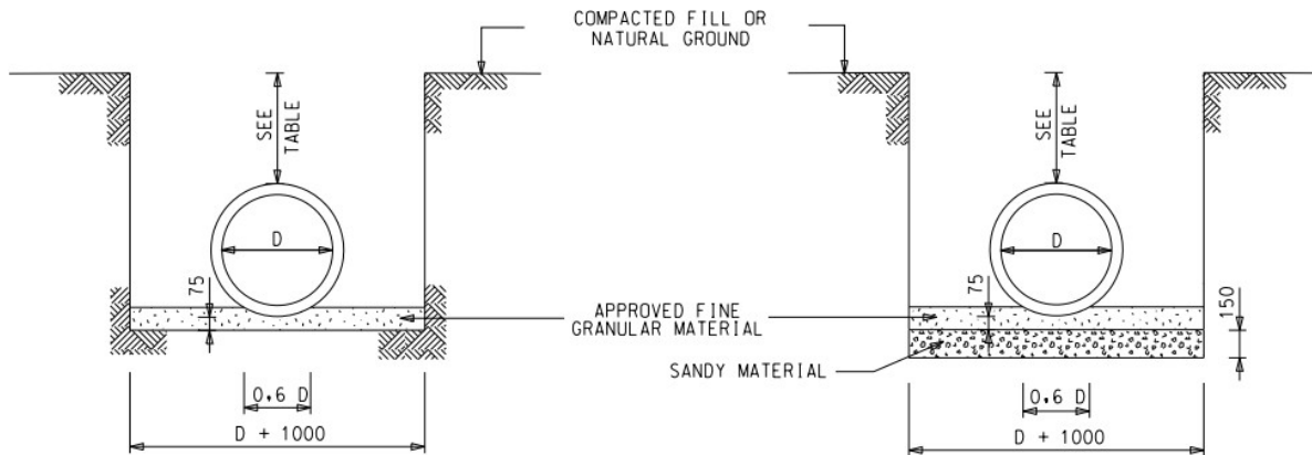
Figure 7. Proposed typical pipe culvert designs in hard material (left) and soft material (right). Source: AURECON (2020).
