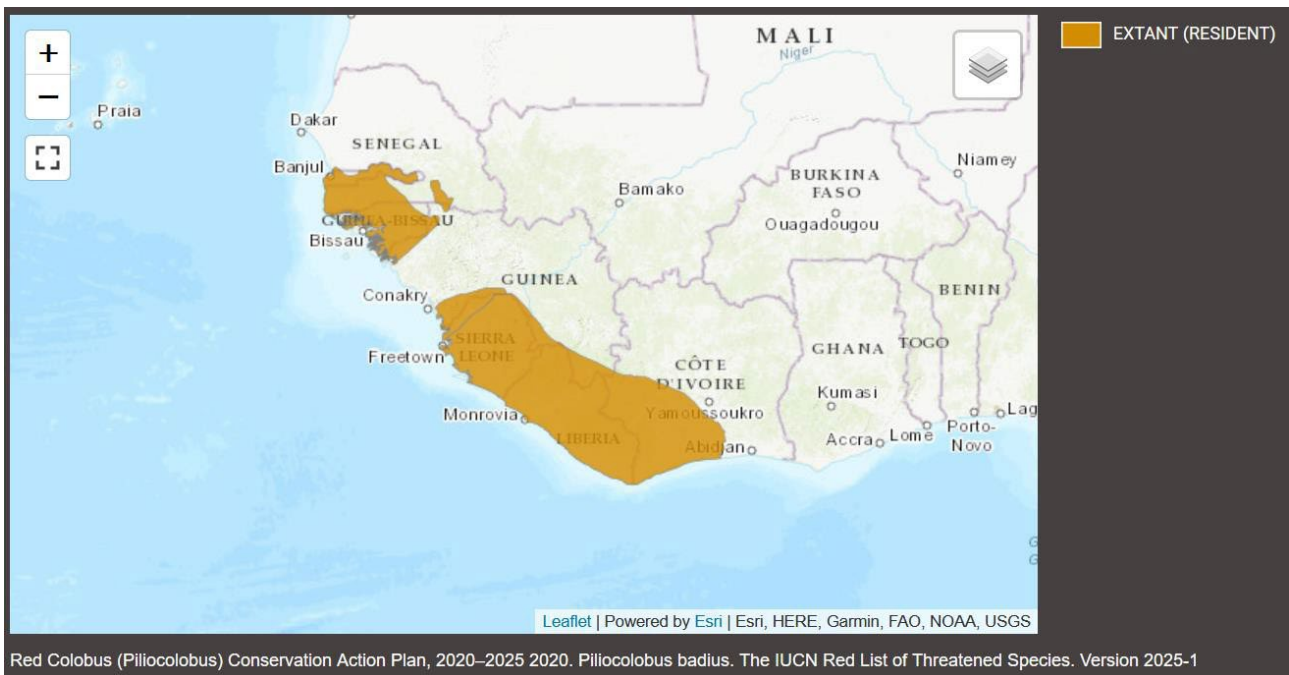
Figure 69. Range of Ptilocolobus badius (IUCN, 2025-I)
