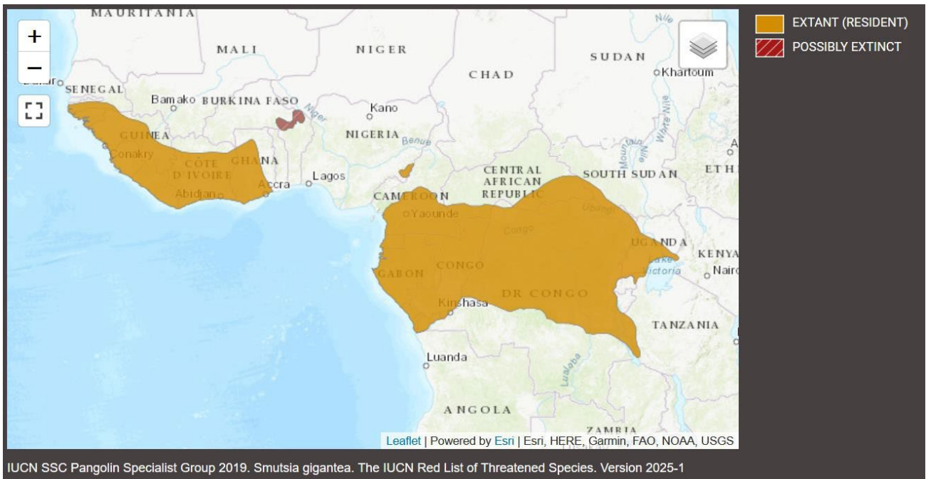
Figure 66. Range of Smutsia gigantea (IUCN, 2025-I)
