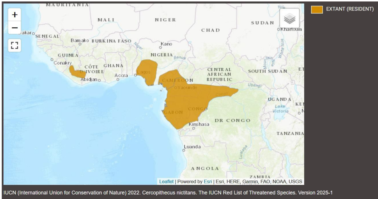
Figure 70. Range of Cercopithecus nictitans (IUCN, 2025-I)
