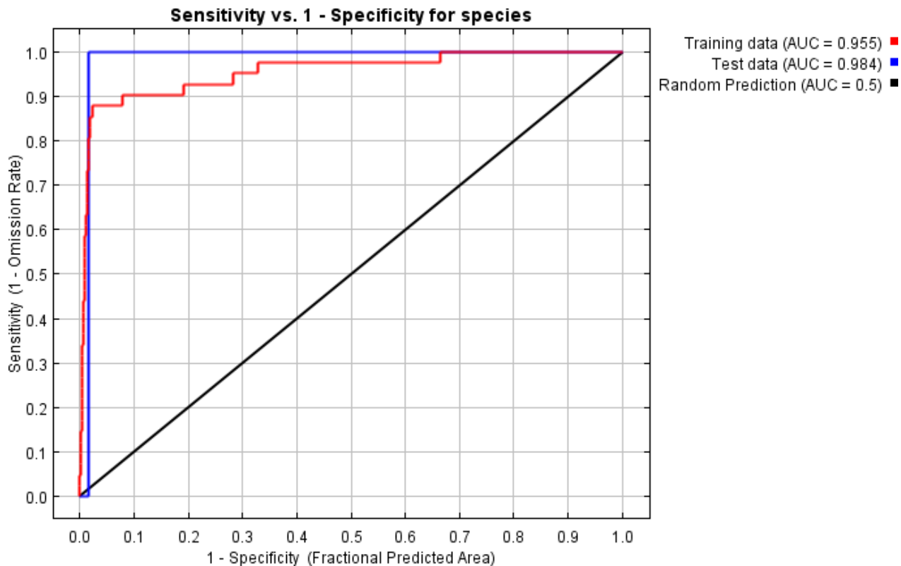
Figure 26. Evaluation results of the climatic habitat suitability of the Giant pangolin in Liberia (FinnOC, 2025)
