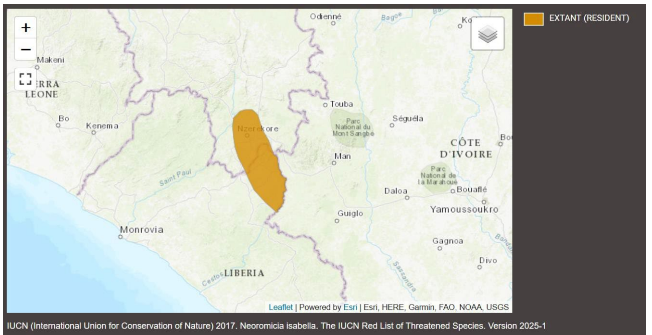
Figure 77. Range of Neoromicia isabella (IUCN, 2025-I)
