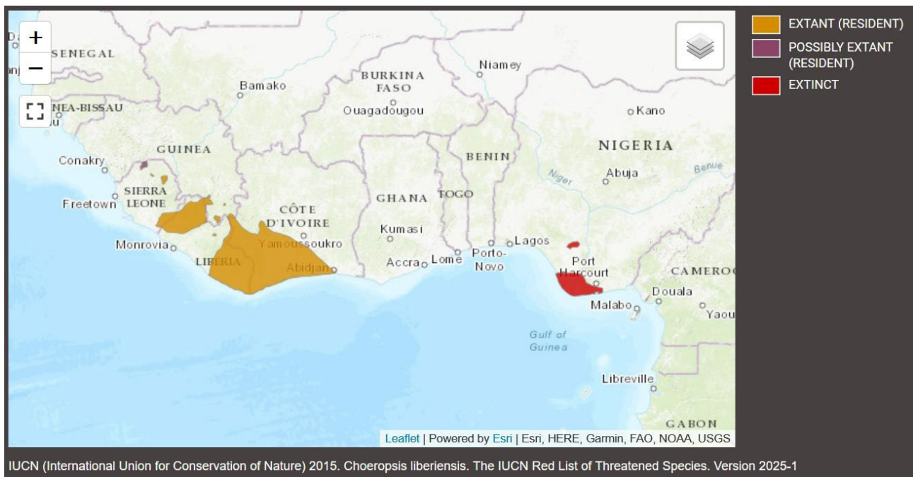
Figure 65. Range of Choeropsis liberiensis (IUCN, 2025-I)
