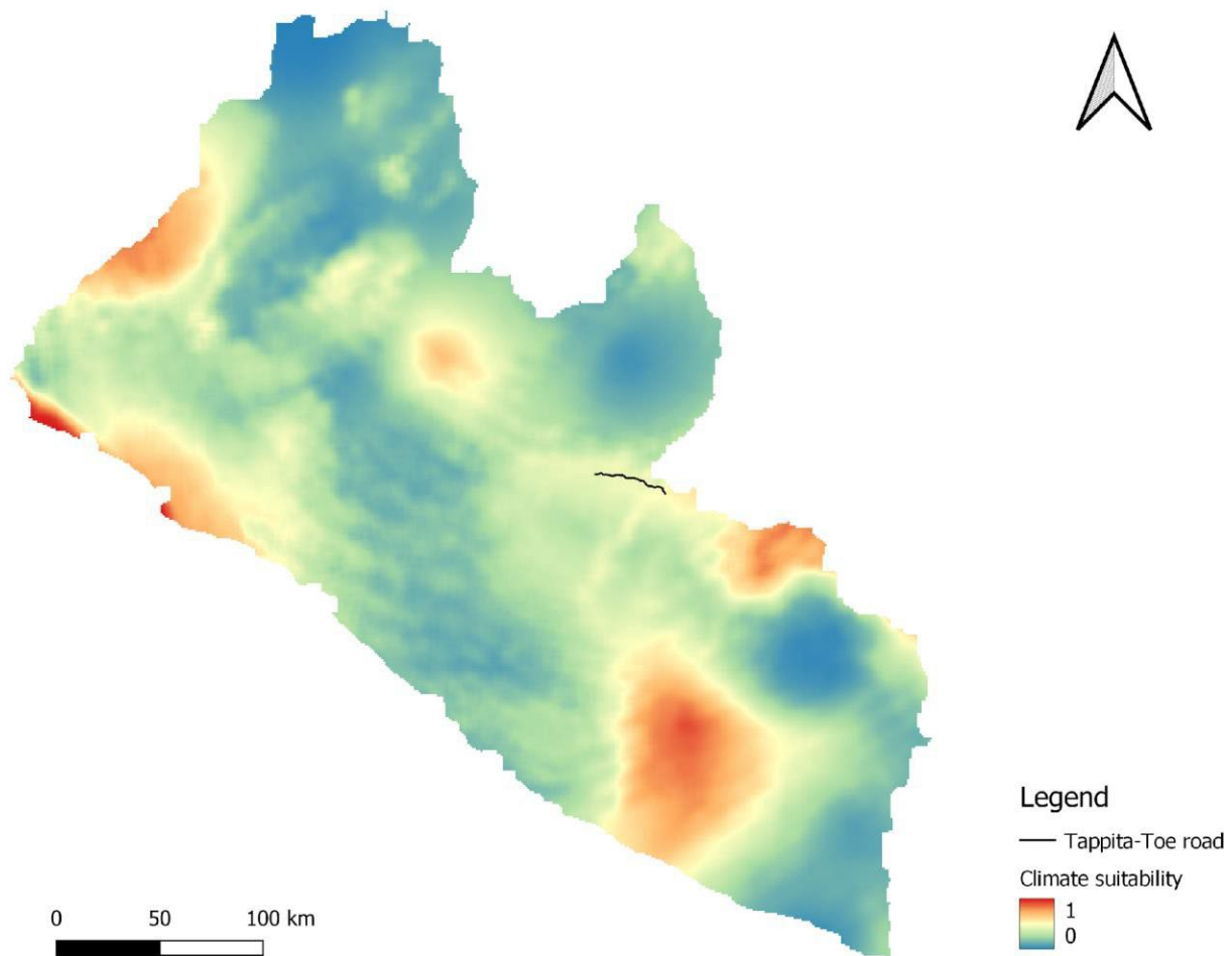
Figure 21. Predicted climatic suitability of Timnhed parrot in Liberia (FinnOC, 2025)
