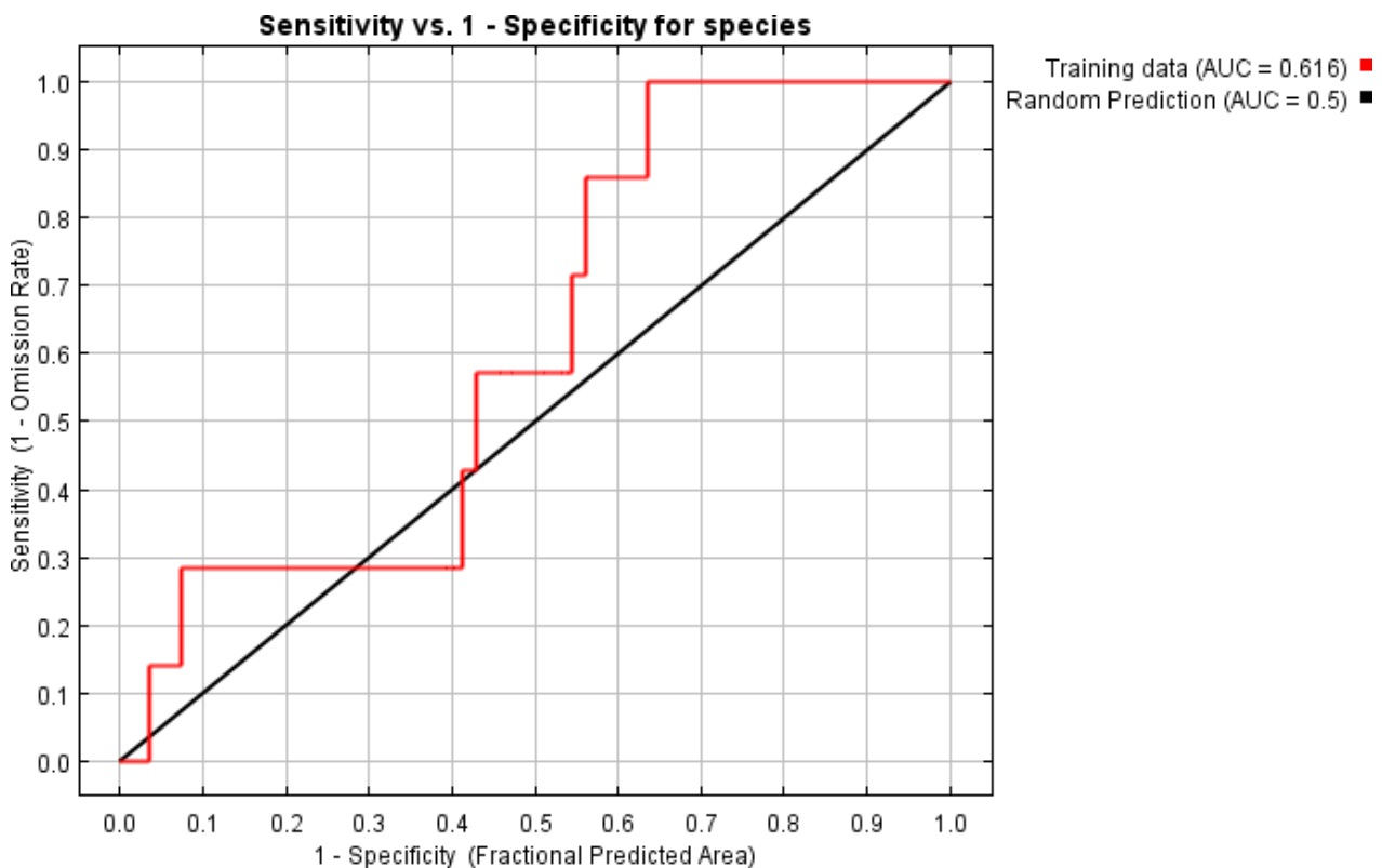
Figure 28. Evaluation results of the climatic habitat suitability of the White-bellied pangolin in Liberia (FinnOC, 2025)
